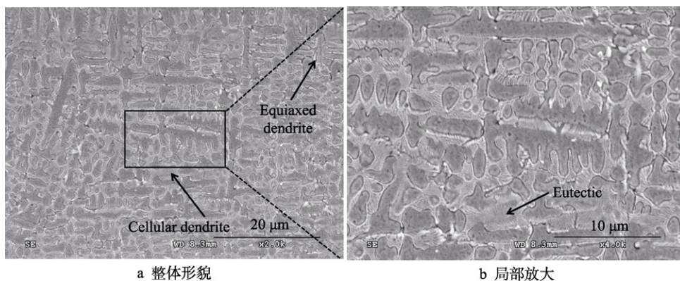
图 6 熔覆层顶部 SEM 形貌 Fig.6 SEM morphology of the top part of the cladding layer: a) overview; b) Local amplification
