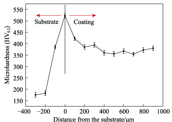
图 8 熔覆层显微硬度分布 Fig.8 Microhardness distribution of cladding layer
