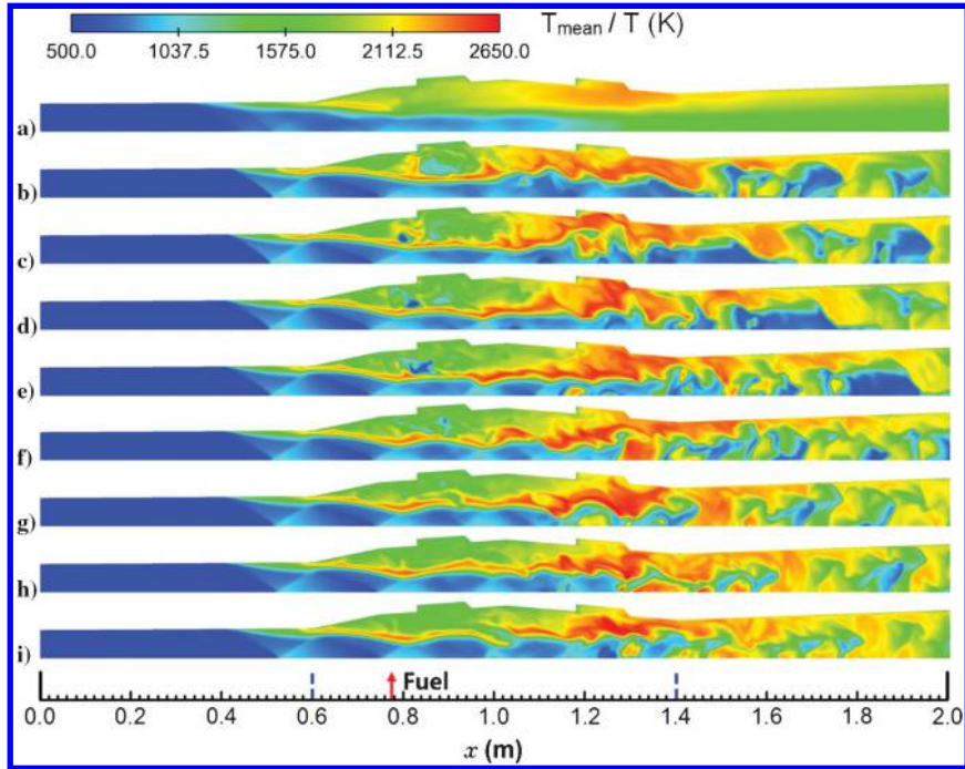
Fig. 14 a) Time-averaged and b–i) instantaneous temperature contours at 0.1 ms intervals on the major axis plane.
