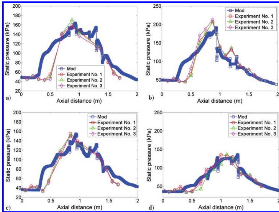
Fig. 5 Comparison of the measured and the predicted time-averaged static pressure for a) the elliptic combustor at Ma = 2.5 , b) the round combustor at Ma = 2.5 , c) the elliptic combustor at Ma = 3.0 , and d) the round combustor at Ma = 3.0 .
