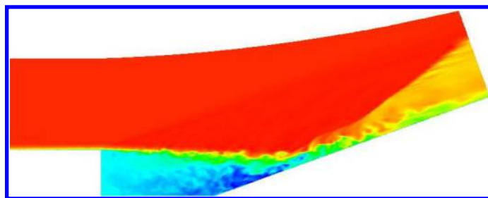
Figure 20. Snapshot of instantaneous streamwise velocity field
