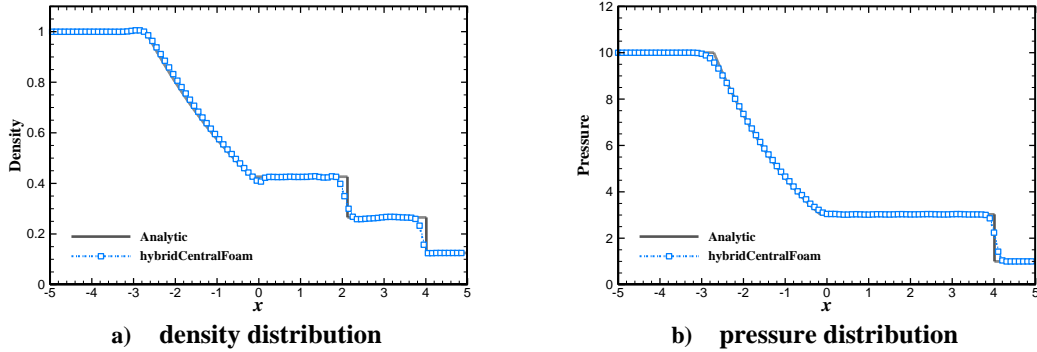
a) density distribution b) pressure distribution Figure 1. Density and pressure profiles for Sod shock tube problem
