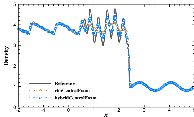
Figure 2. Density profiles for Shu-Osher problem (200 points)
