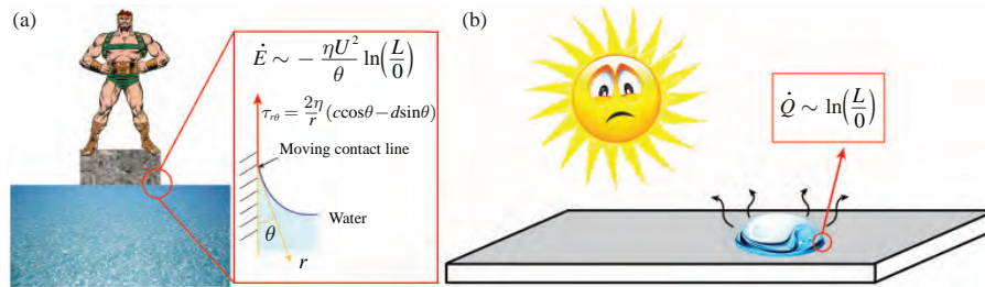
Fig. 1. The two paradoxes in MCL problem: (a) Huh–Scriven paradox and (b) droplet evaporation paradox.
