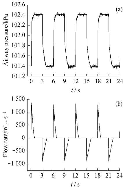
图2 与呼吸模拟器 ASL 5000 连接的呼吸机上监测得到的压力 (a) 和流量 (b) 曲线 Fig.2 Pressure (a) and flux (b) curves monitored by the ventilator connected with ASL 5000 breathing simulator
