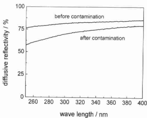
Fig. 3 Comparison of the diffusive reflectivity of MgF 2 coating surface before and after contaminated by N 2 O 4 vapor at the pressure of 6.9 \times 10^4 Pa
