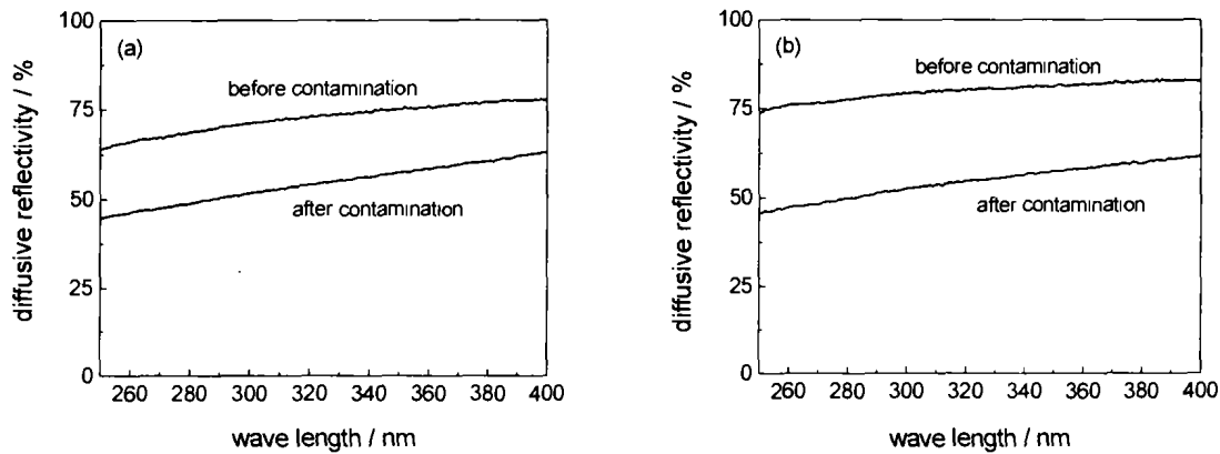
Fig. 4 Comparison of the diffusive reflectivity of MgF_2 coating surface before and after contaminated by solid particles of N_2O_4 (a) No.1 sample (b) No.2 sample
