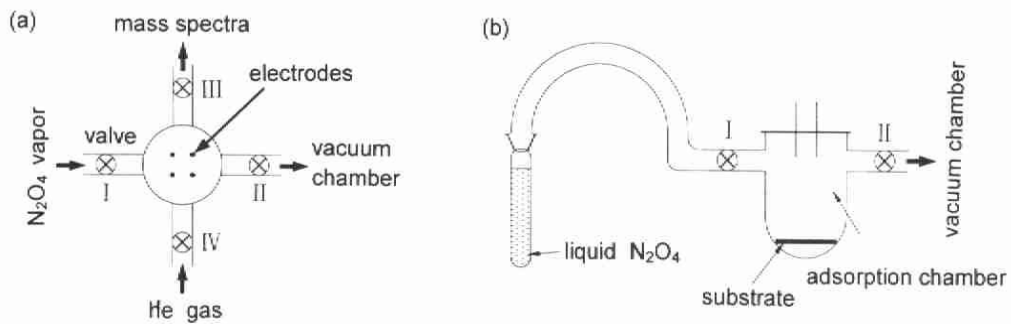
Fig. 2 Top view (a) and side view (b) of an experimental device for contamination of diffusively reflecting flakes by N 2 O 4
