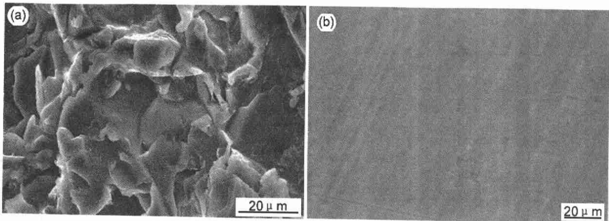
Fig. 1 Surface morphology of a diffusively reflecting flake. (a) MgF 2 coating; (b) aluminum substrate
